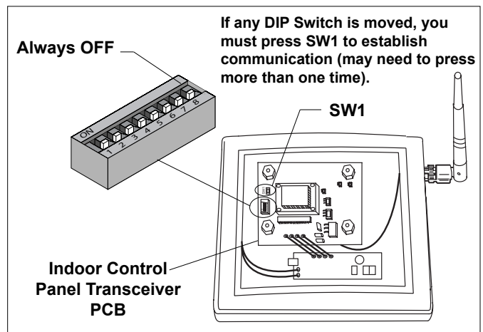
Figure 32. DIP Switch Settings at Wireless Indoor Control Panel
