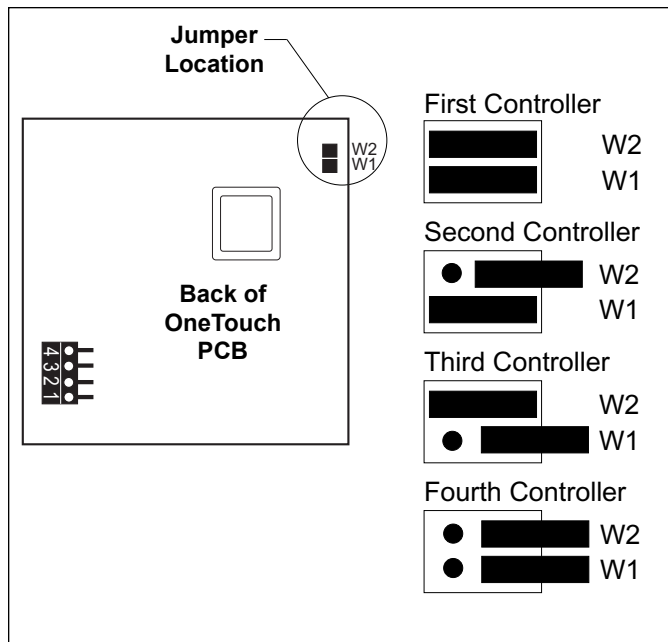
Figure 29. Jumper Settings for Multiple OneTouch Control Panels
