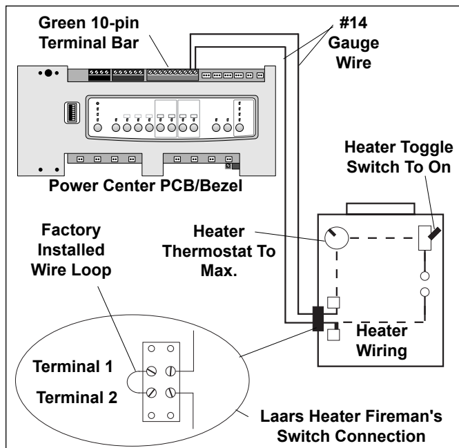
Figure 9. Laars Heater Connection
